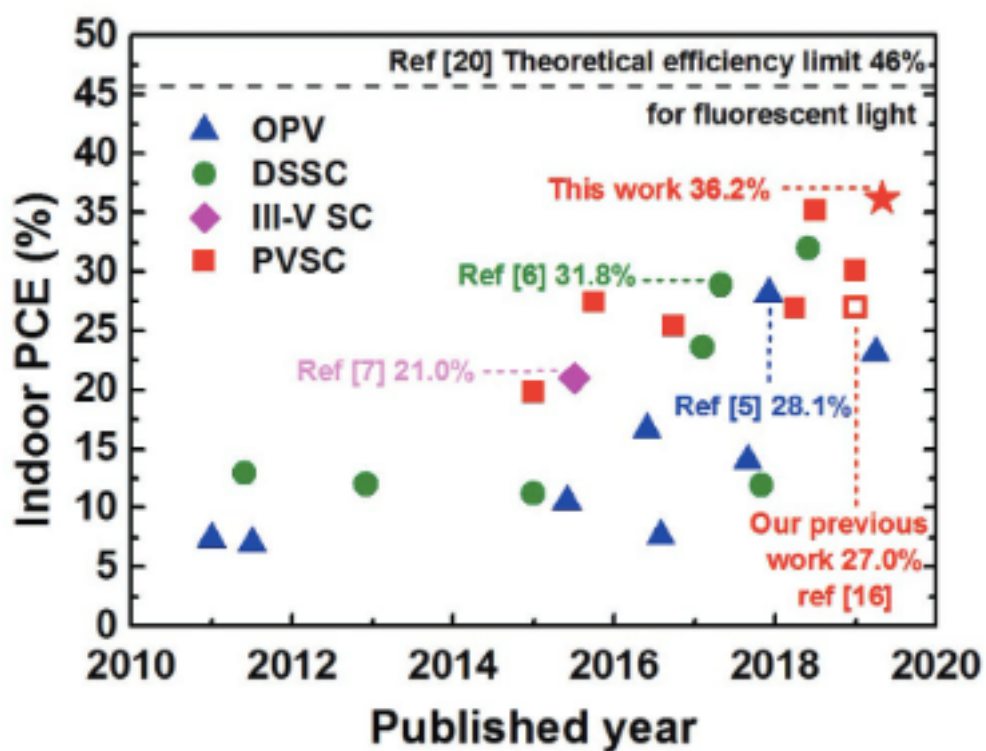
Figure 5. Summarized indoor PCE of representative works of OPV, DSSC, III-V SC, and PVSC.
